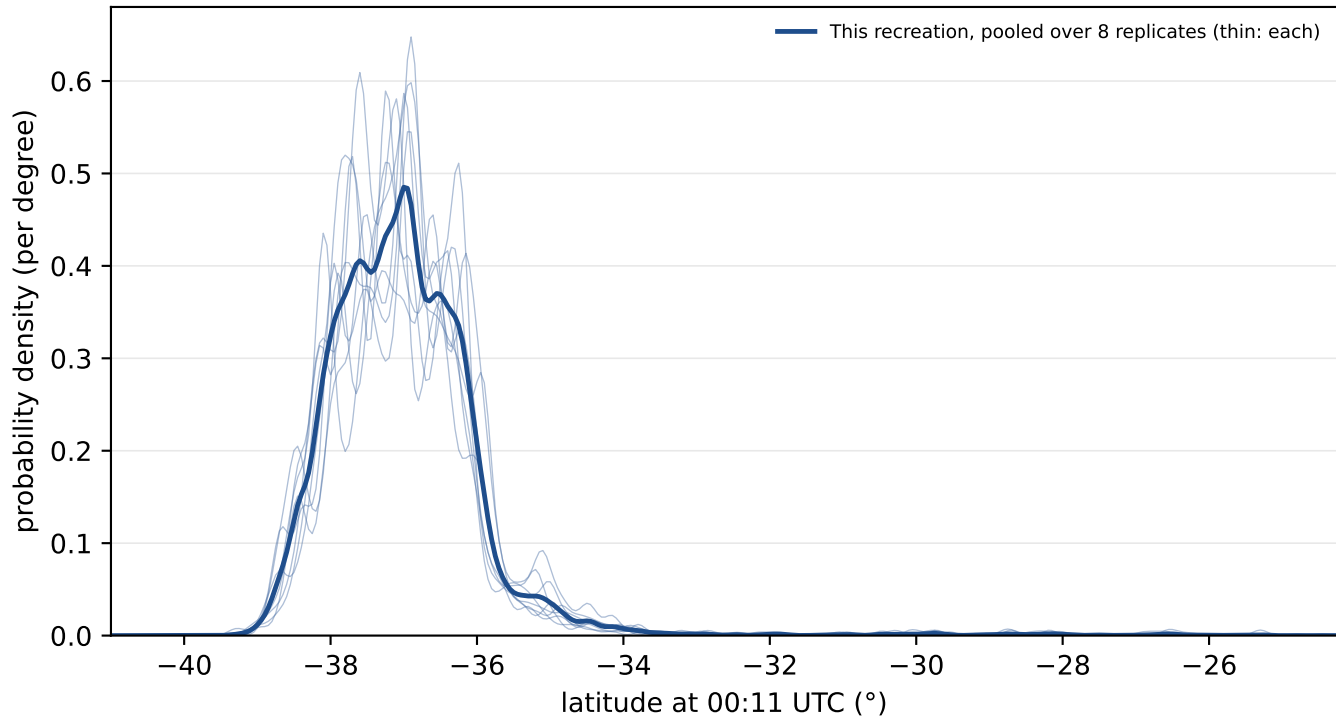
Latitude pdf at 00:11 UTC — tempered-three
